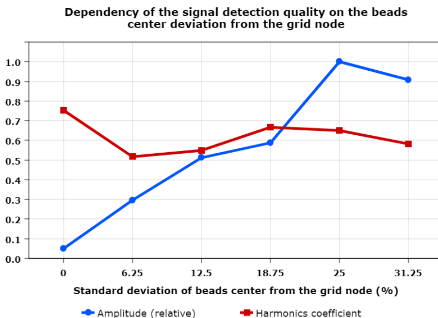
Fig. 10. – Dependency of the signal detection quality on the bead center deviation from the grid node
