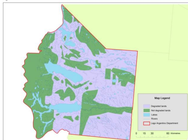
Figure 3. Results of composite image decoding.
