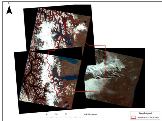
Figure 1. Scheme of Landsat 7 images decoding in 2001
