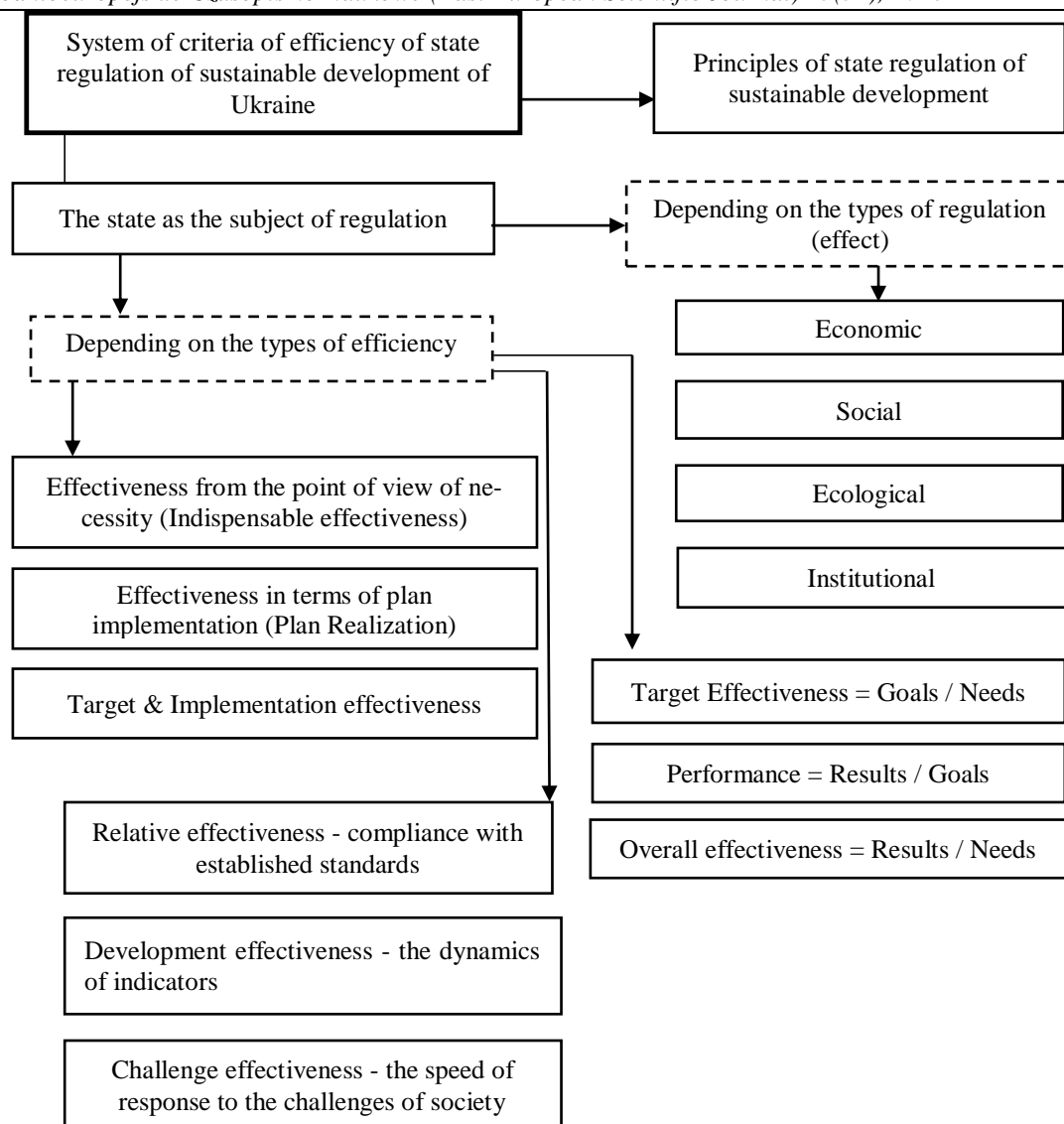
Fig. 1. The system of criteria for evaluating the effectiveness of the state regulation of sustainable development of Ukraine
