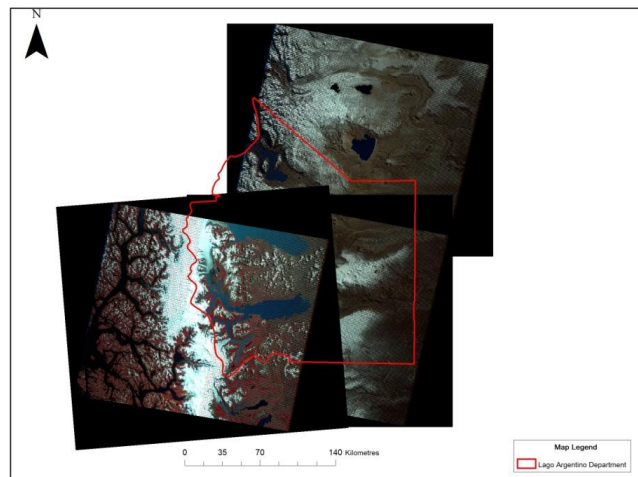
Figure 2. Scheme of Landsat 7 decoding for 2012.
