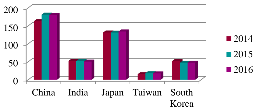
Figure 2. Consumption of natural gas, ppb. cube. m. Source: [3]
