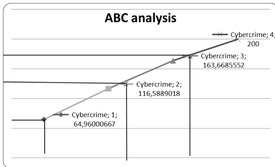
Figure 4 – Graphic result of ABC analysis
