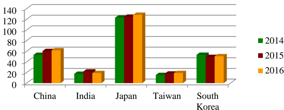
Figure 1. Natural gas imports from ATP countries to Australia and the Far East, ppb. m. Source: [3]
