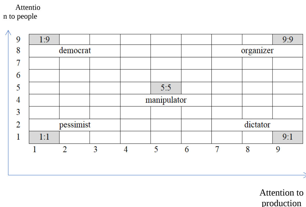
Fig.1. Blake-Mouton Grid
