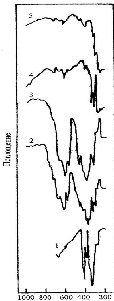
Fig.4. IR-spectrum of alloys of the system La_2S_3 - Ga_2S_3 - Sm_2S_3
